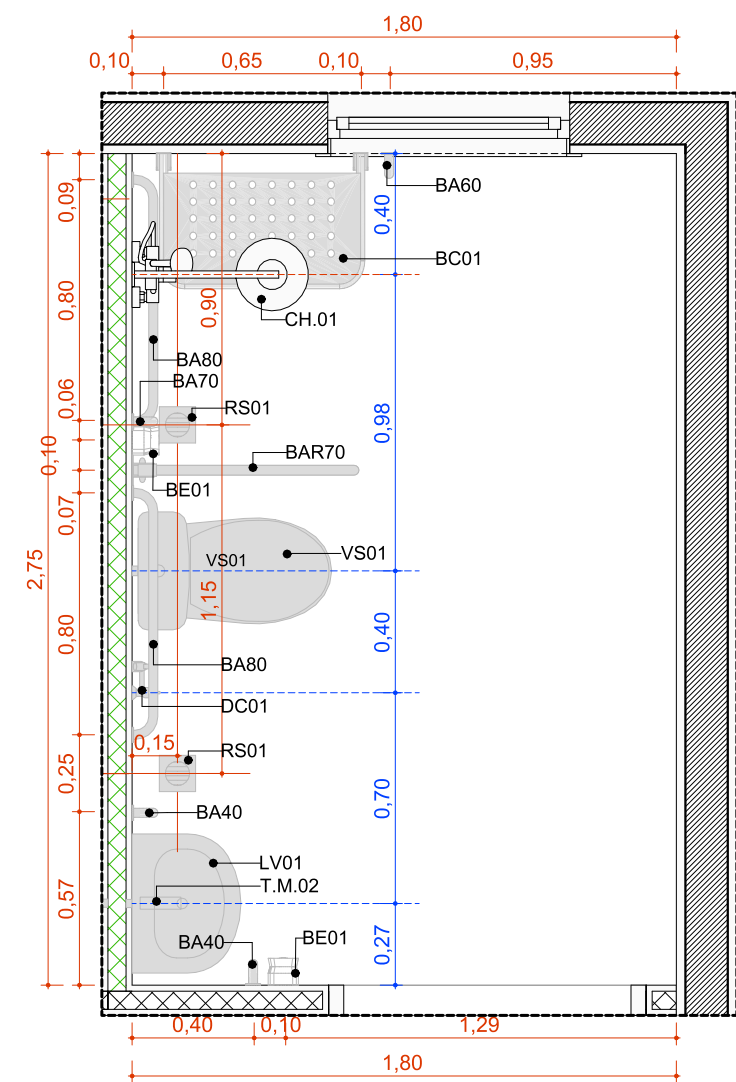
A.M.10 Banh. PCD Func. Escala:1:25
